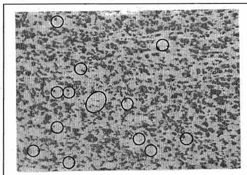
Figure 7: Optical micrograph of Composite 2 specimen in S-T direction (100 x).
