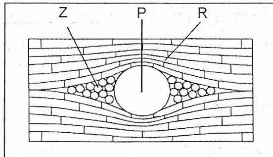
Figure 10: Schematic diagram should the rotated deformation zones and the distortions associated with large particles (7) ; Z, P and R indicate a rotated zone, a particle and a distorted zone respectively.
